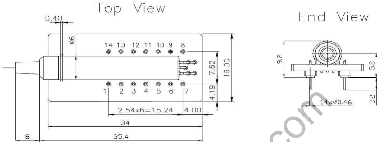
Package Type A
